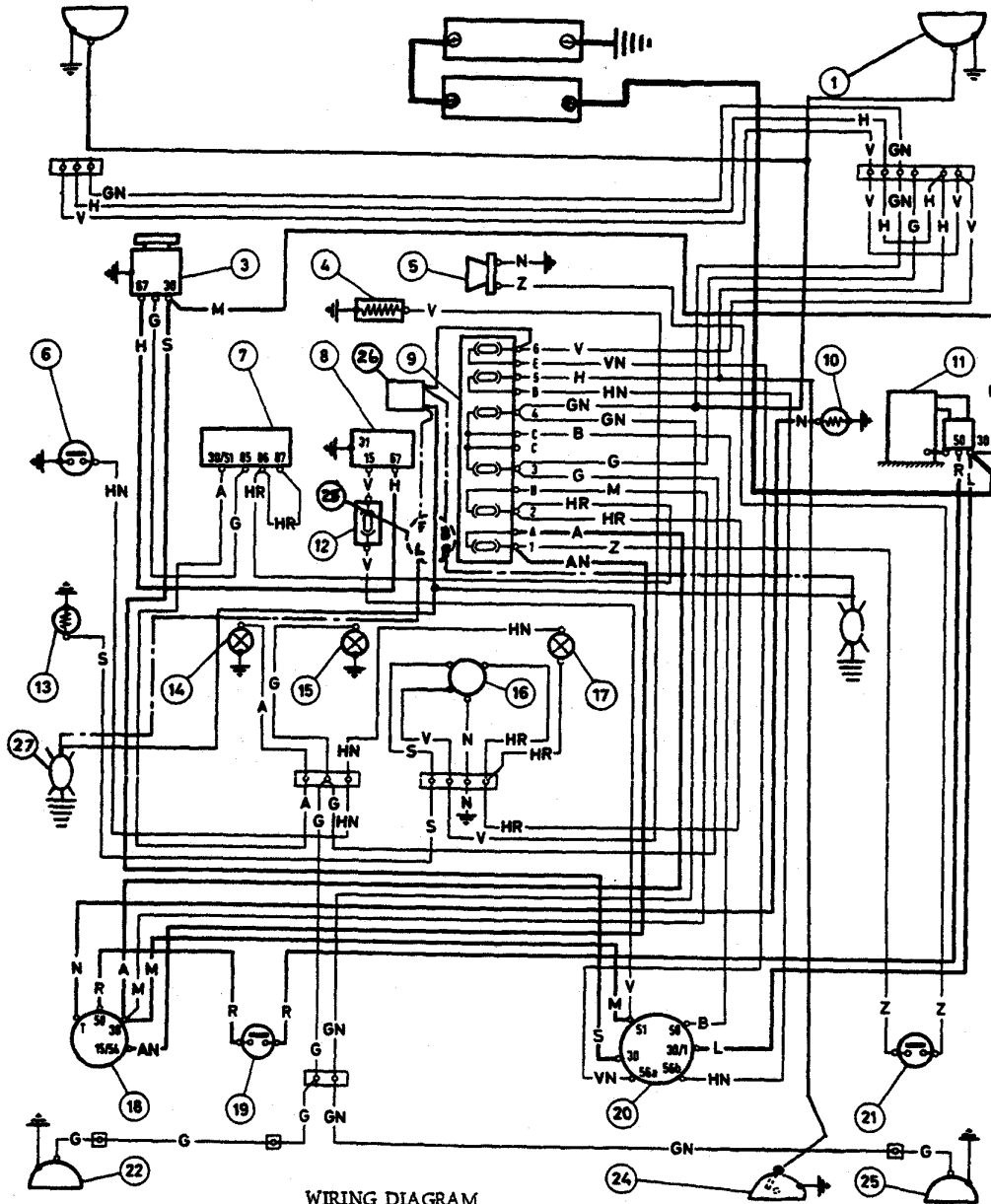
WIRING DIAGRAM
