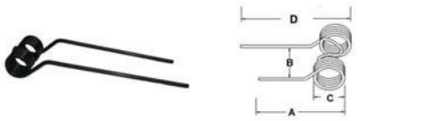
A-51000856 Tedder Tooth (LH)
