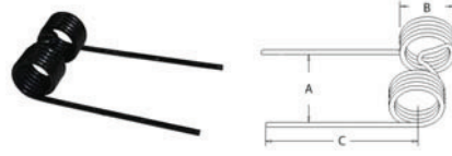
A-7895642 Tine, Double
