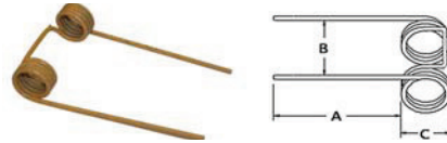
A-37762 Baler Tooth
