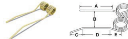
A-51001367 Tedder Tooth
