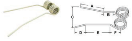
A-PZ110 Tedder Tooth
