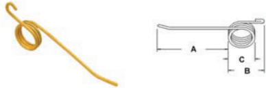
A-NE400033 Rake Tooth
