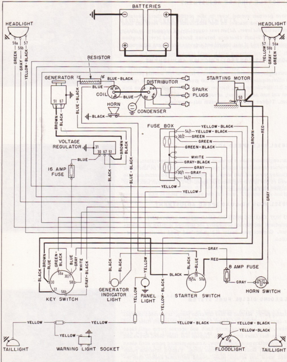
Gasoline Wiring Diagram
