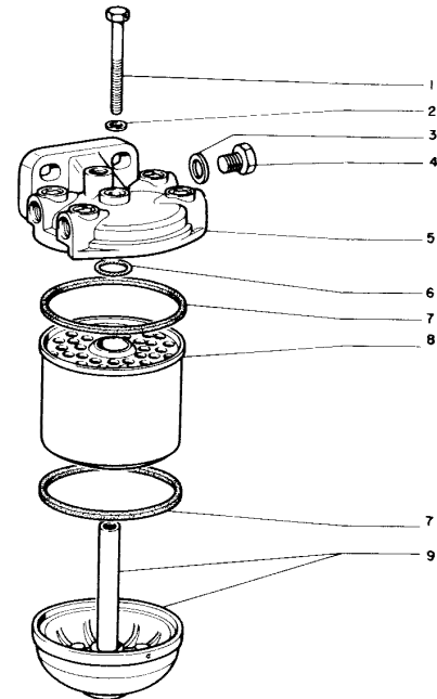
676951AS Assembly
