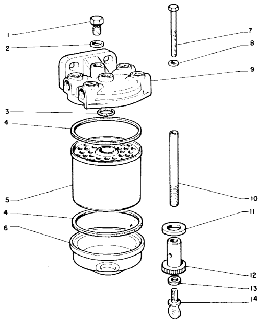
676949AS Assembly
